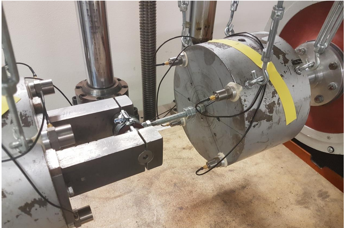
Figure 1. Test configuration (exemplary).
